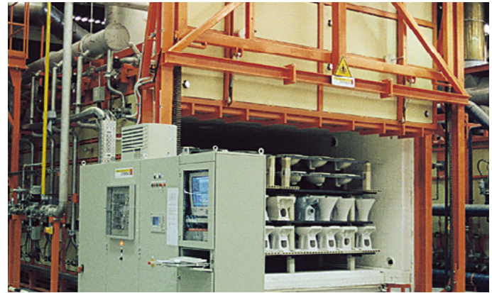
Intermittent shuttle kiln in the ceramics industry
